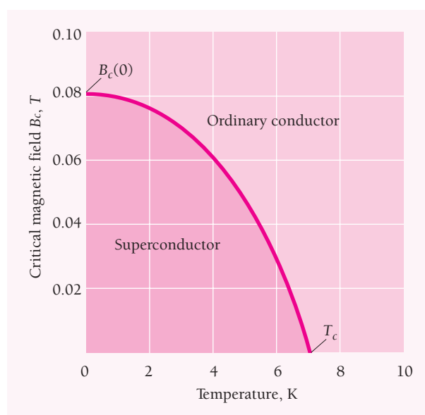
Figure 10.50 Variation of the critical magnetic field B_c with temperature for lead. Below the curve, lead is a superconductor; above the curve, it is an ordinary conductor.
