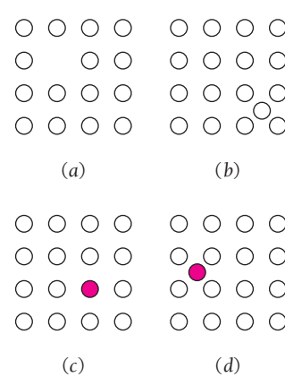
Figure 10.2 Point defects in a crystal. (a) Vacancy. (b) Interstitial. (c) Substitutional impurity. (d) Interstitial impurity.
