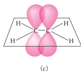
Figure 8.14 (a) The ethylene ( C_2H_4 ) molecule. All the atoms lie in a plane perpendicular to the plane of the paper. (b) Top view, showing the sp^2 hybrid orbitals that form \sigma bonds between the C atoms and between each C atoms. (c) Side view, showing the pure p_x orbitals that form a \pi bond between the C atoms.
