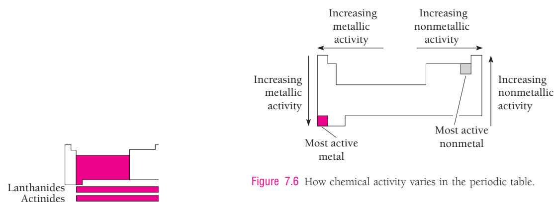
Figure 7.7 The transition elements are metals.
