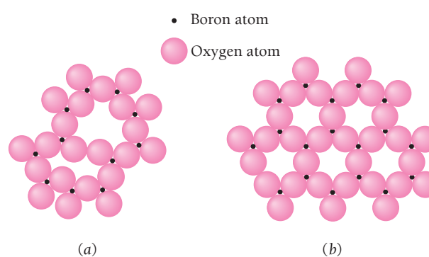
Figure 10.1 Two-dimensional representation of \text{B}_2\text{O}_3 . (a) Amorphous \text{B}_2\text{O}_3 exhibits only short-range order. (b) Crystalline \text{B}_2\text{O}_3 exhibits long-range order as well.
