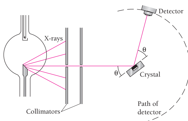
Figure 2.21 X-ray spectrometer.
