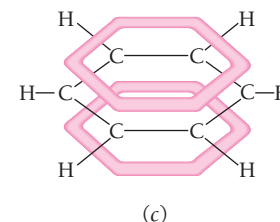
Figure 8.15 The benzene molecule. (a) The overlaps between the sp^2 hybrid orbitals in the C atoms with each other and with the s orbitals of the H atoms lead to \sigma bonds. (b) Each C atom has a pure p_x orbital occupied by one electron. (c) The bonding \pi molecular orbitals formed by the six p_x atomic orbitals constitute a continuous electron probability distribution around the molecule that contains six delocalized electrons.
