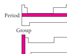
Figure 7.4 The elements in a group of the periodic table have similar properties, while those in a period have different properties.
