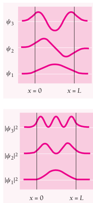
Figure 5.8 Wave functions and probability densities of a particle in a finite potential well. The particle has a certain probability of being found outside the well.
