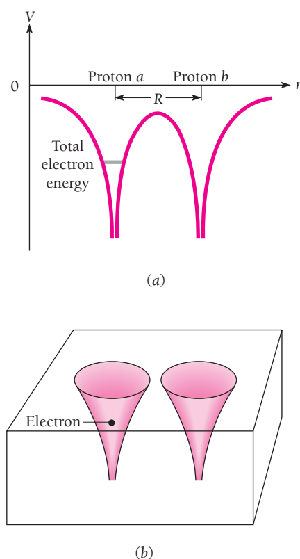
Figure 8.4 (a) Potential energy of an electron in the electric field of two nearby protons. The total energy of a ground-state electron in the hydrogen atom is indicated. (b) Two nearby protons correspond quantum-mechanically to a pair of boxes separated by a barrier.
