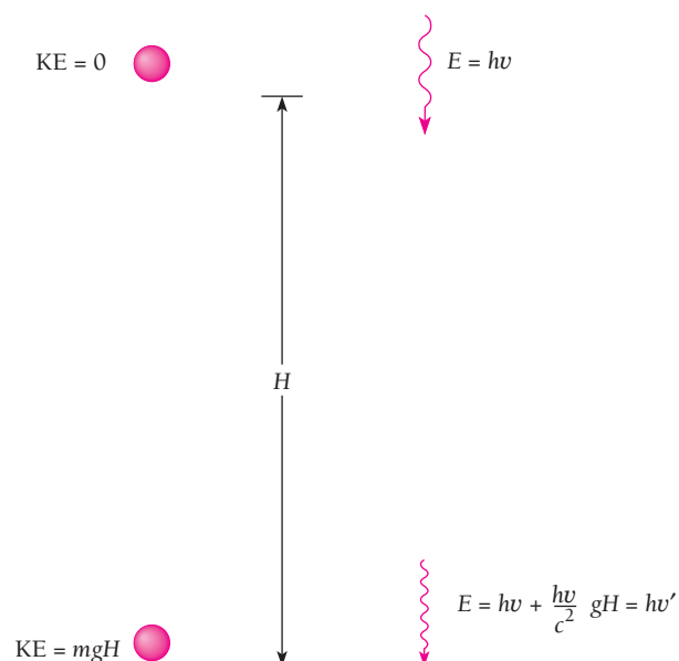
Figure 2.30 A photon that falls in a gravitational field gains energy, just as a stone does. This gain in energy is manifested as an increase in frequency from \nu to \nu' .
