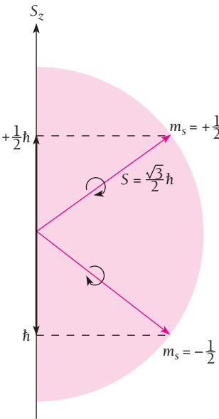
Figure 7.2 The two possible orientations of the spin angular-momentum vector are “spin up” ( m_s = +\frac{1}{2} ) and “spin down” ( m_s = -\frac{1}{2} ).
